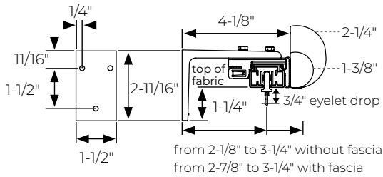
R-TEC Single Motorized Bracket TB035-R
