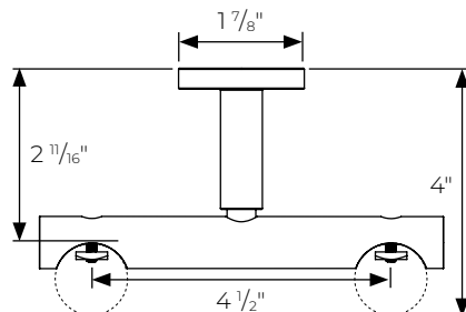
Ceiling Mount Double PTHMT138404
