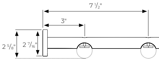
Wall Mount Double PTHMT138402
