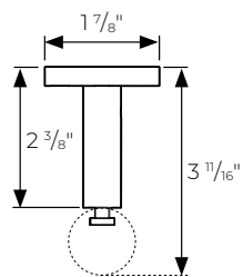
Ceiling Mount Single PTHMT138403
