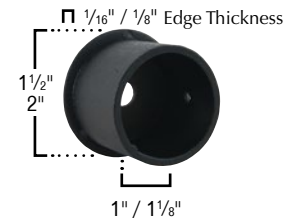
303 Socket (New!) (For 1" & 1½" Rods)
