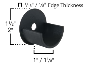
302 Socket (New!) (For 1" & 1½" Rods)
