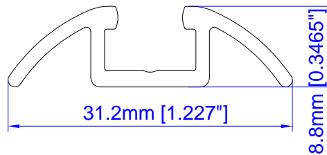
M Shape Bottom Track
