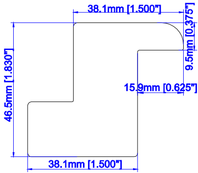
1 1/2" Bullnose Z Frame
