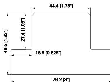
1.75" Chamfer T Post with 3/4" Light Block (L/Z/HS)
