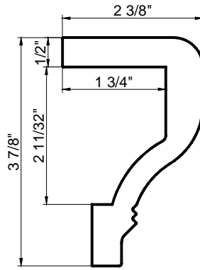
Designer Sill Cap (D/HS)
