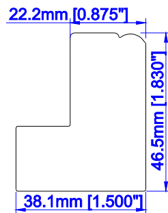
2" Bel Air Z Sill Plate
