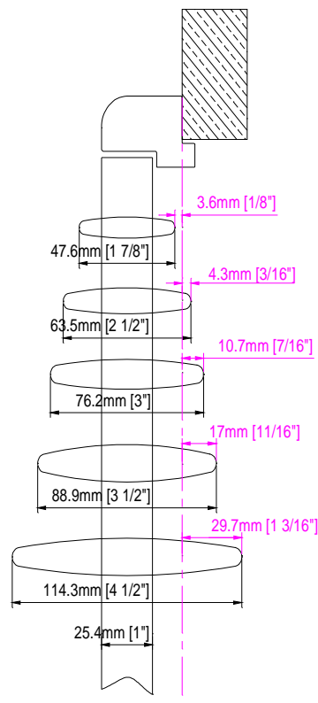
Tilt Out Z Frame
