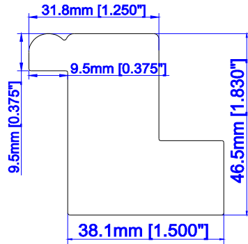
1 1/4" Beaded Z Frame
