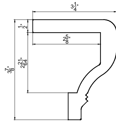
Designer Sill Cap (Z)
