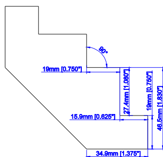
Corner Post with 3/4" Light Block (L/Z/HS)
