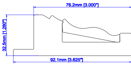
3" Ridge Deco Frame
