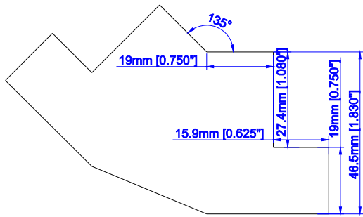
Bay Post with 3/4" Light Block (L/Z/HS)
