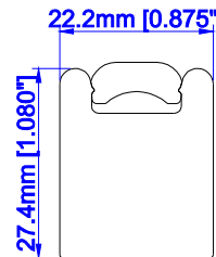
7/8" Vintage Hang Strip
