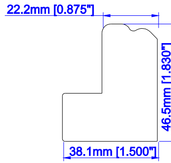
3" Crown Z Sill Plate
