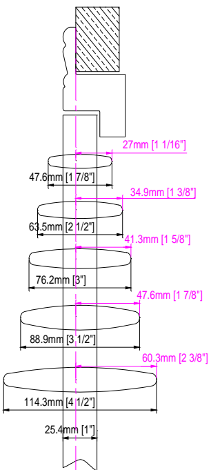
2" Bel Air Z Frame
