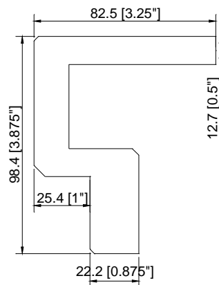
Mission Sill Cap (Z)
