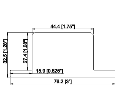
1.75" Chamfer T Post with 1/4" Light Block (Deco)
