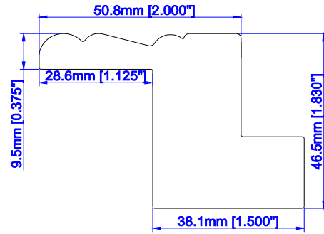
2" Bel Air Z Frame
