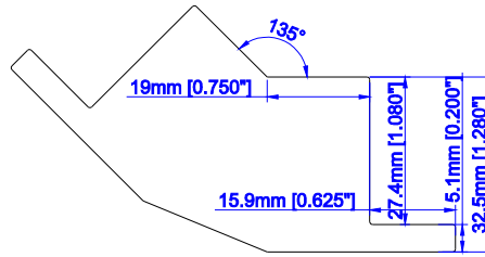
Bay Post with 1/4" Light Block (Deco)
