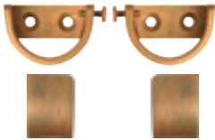
IM125 1 1/4" steel inside mount brackets 1 1/8"H x 1 3/8"W backplate, 3/4" Deep, 1/8" thick backplate per bracket (sold in pairs)
