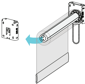
Attach Clutch, swing assembly to bracket
