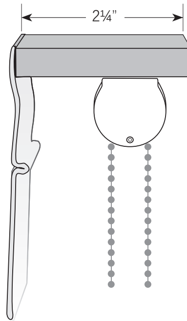
MANUAL CHAIN HEAD RAIL
