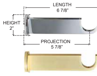
ACBRE-138-E 1 3/8" DIA EXTENDED SINGLE METAL BRACKET
