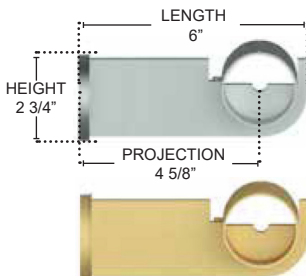
ACBRJ-218-S 2 1/8" DIA STANDARD SINGLE METAL JOINING BRACKET
