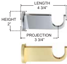
ACBRE-138-S 1 3/8" DIA STANDARD SINGLE METAL BRACKET
