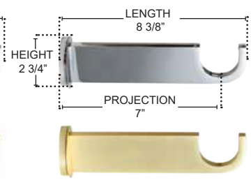
ACBRE-218-E 2 1/8" DIA EXTENDED SINGLE METAL BRACKET
