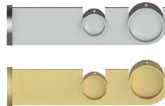
ACBRD-J DOUBLE METAL JOINING BRACKET 1 3/8" BACK, 2 1/8" FRONT
