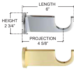
ACBRE-218-S 2 1/8" DIA STANDARD SINGLE METAL BRACKET
