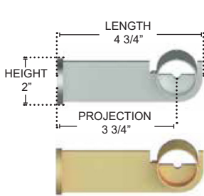
ACBRJ-138-S 1 3/8" DIA STANDARD SINGLE METAL JOINING BRACKET
