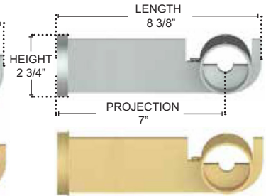
ACBRJ-218-E 2 1/8" DIA EXTENDED SINGLE METAL JOINING BRACKET
