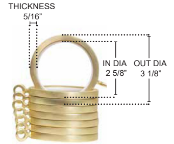
ACRL-218-7 METAL RING WITH NYLON LINER SET OF 7 for 2 1/8" DIA pole
