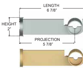
ACBRJ-138-E 1 3/8" DIA EXTENDED SINGLE METAL JOINING BRACKET
