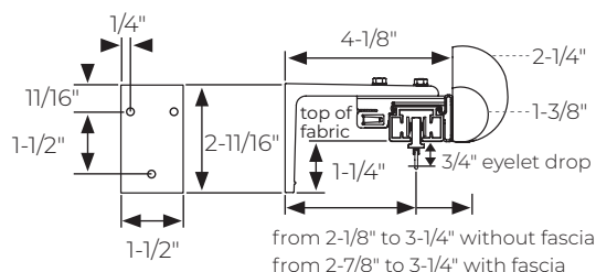
R-TEC Single Motorized Bracket TB035-R
