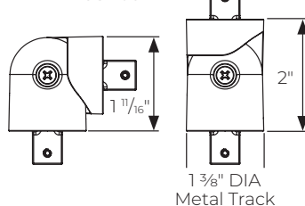
Hinged Elbow PTHMT138409
