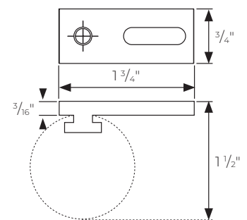
Ceiling Bracket Extender PTHMT138405
