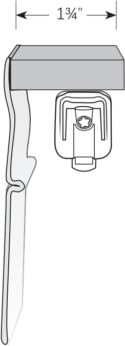
MANUAL CORDLESS HEAD RAIL
