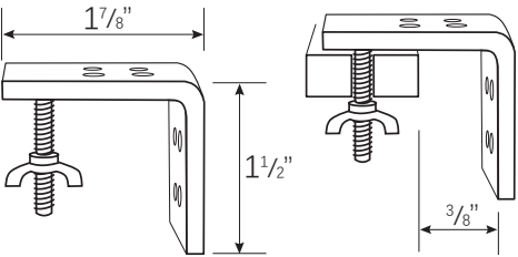
MANUAL CORDLESS BRACKET
