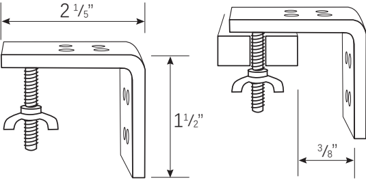
CHAIN BRACKET/ MOTORIZED CORDLESS BRACKET
