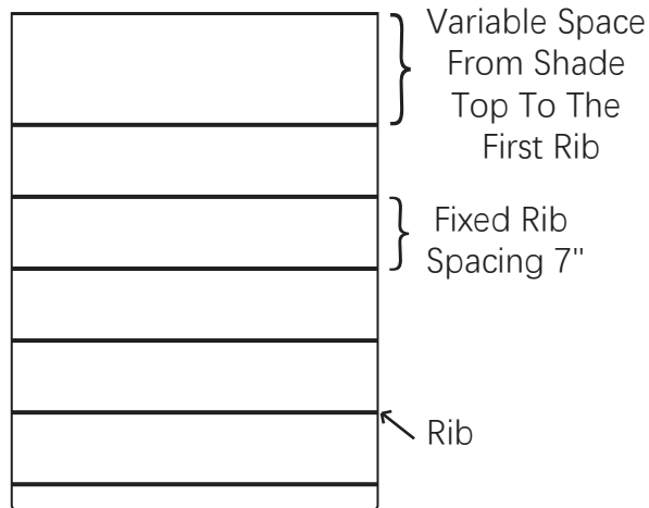
THE SHADE IS PULLED DOWN (FRONT VIEW)
